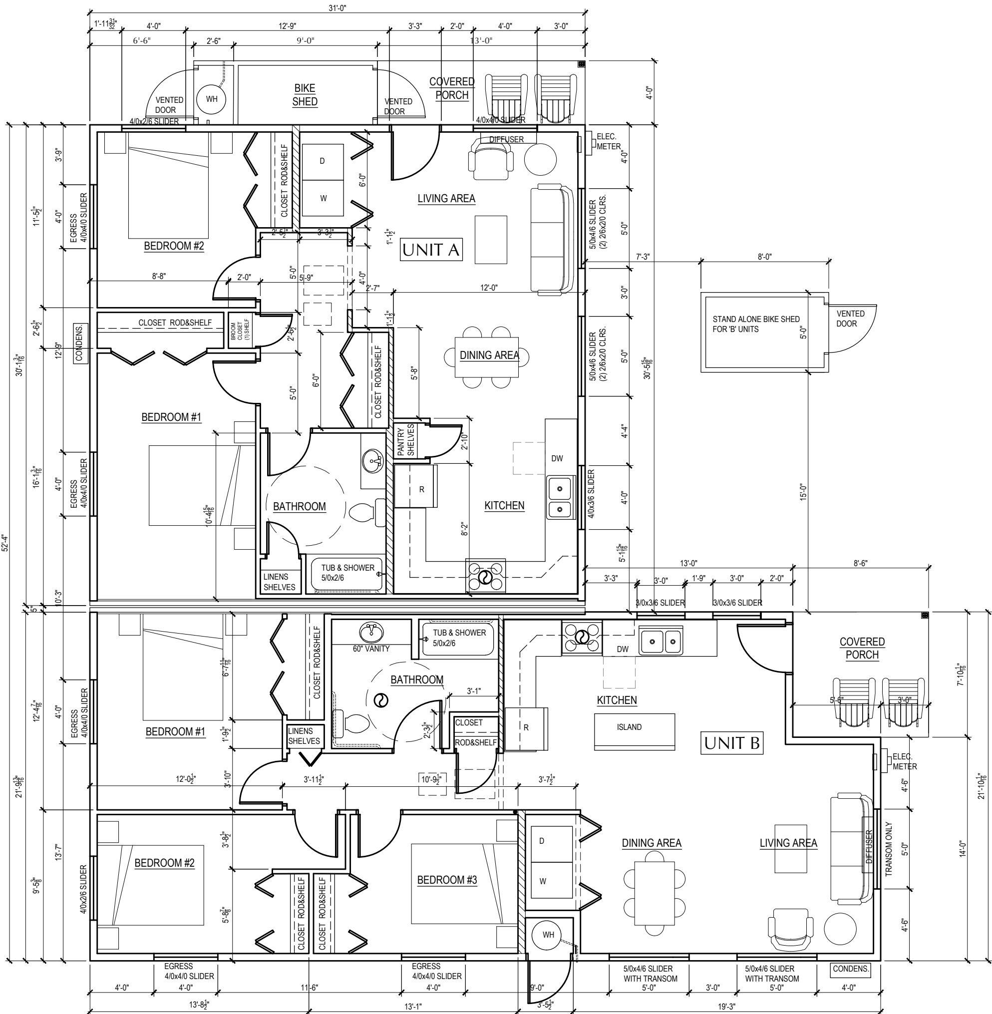
FLOOR PLAN - DUPLEX 4, 5, 6 AND 7
